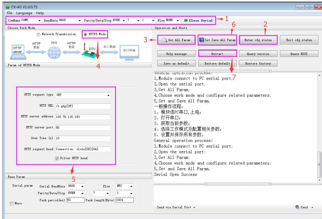
Diagram 5 setting software
